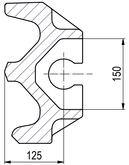
N-N (1:5)
