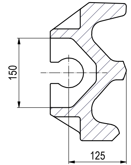
P-P (1:5)
